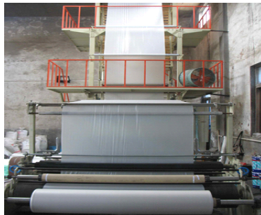
Film Blowing
